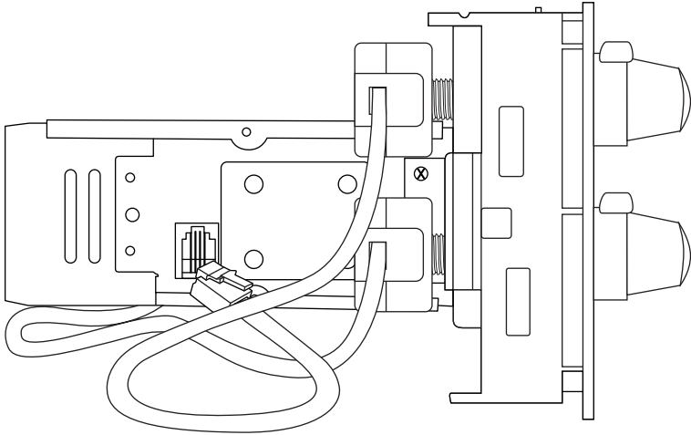
Figure 1 - Ensure Shafts are Plugged In
