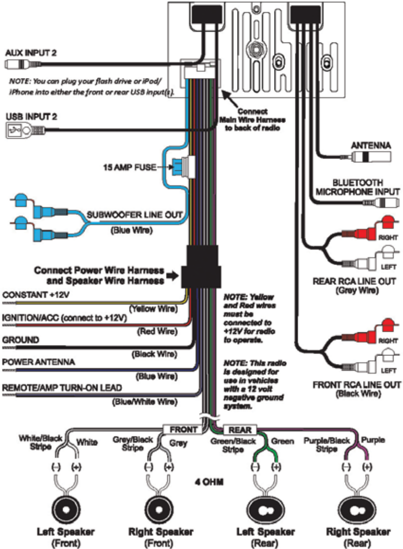
Figure 2 - Wiring Diagram
