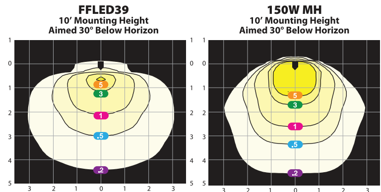
Multiples of Mounting Height - Values shown in Footcandles
