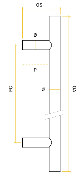
GUARDSMAN PULL HANDLE
