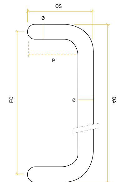
CRANKED PULL HANDLE
