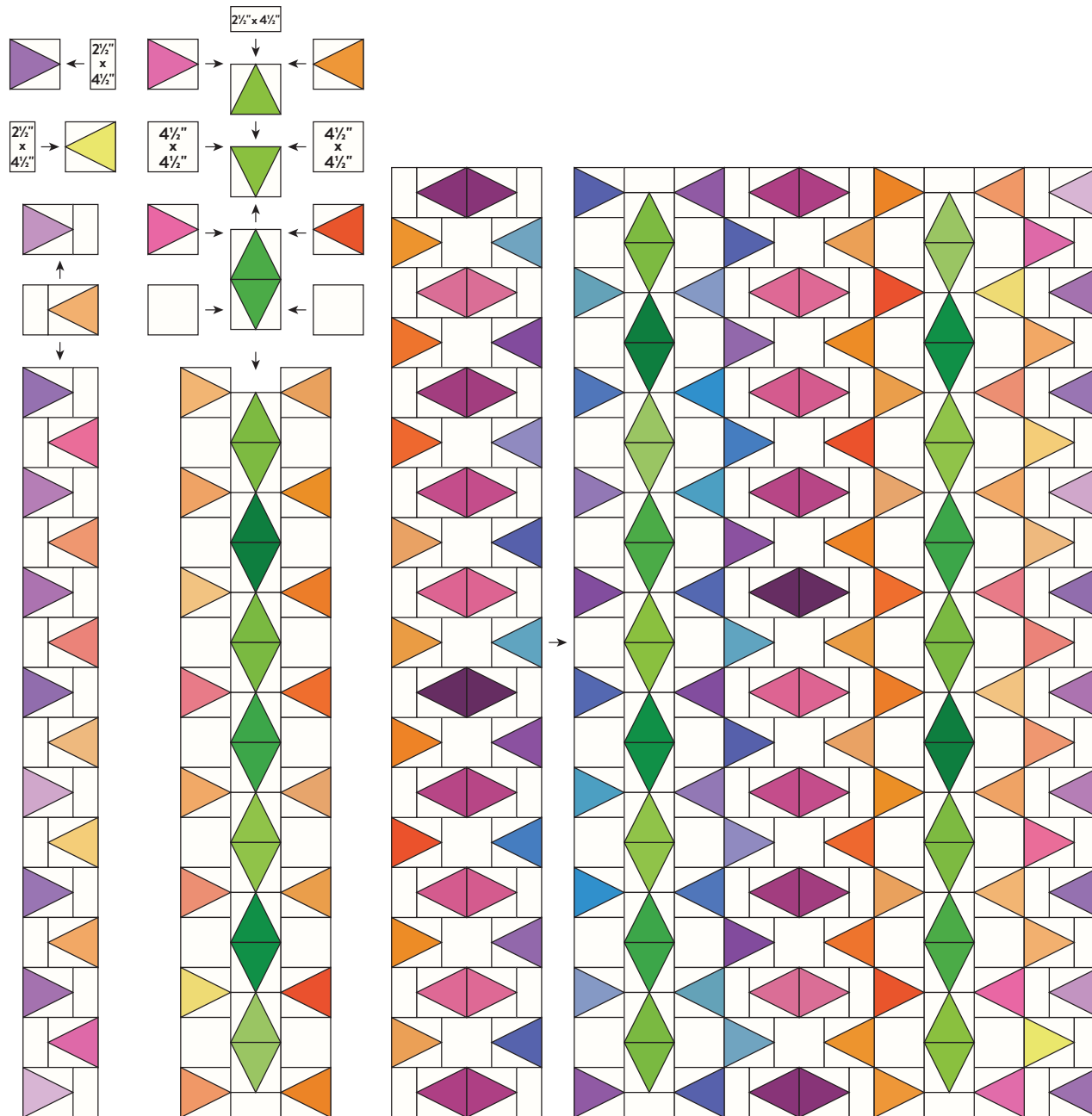
Triangle-in-a-Square Diagram 1
