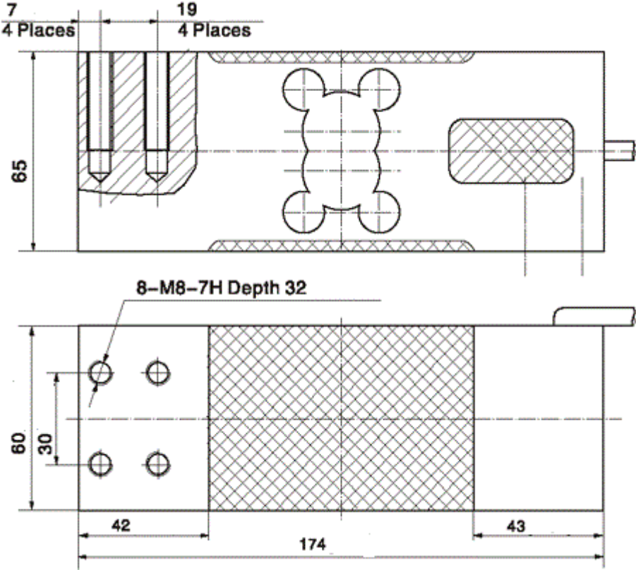
Dimensions (mm)
