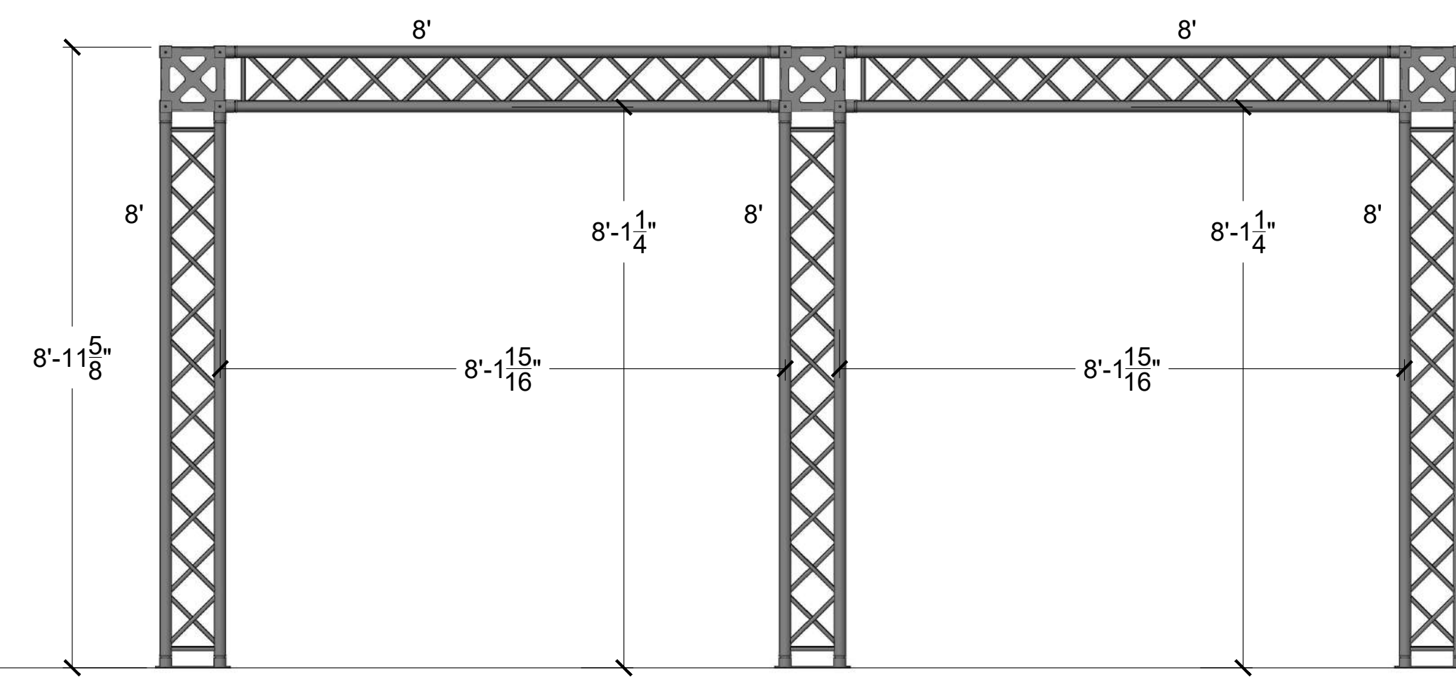
FRONT ELEVATION
