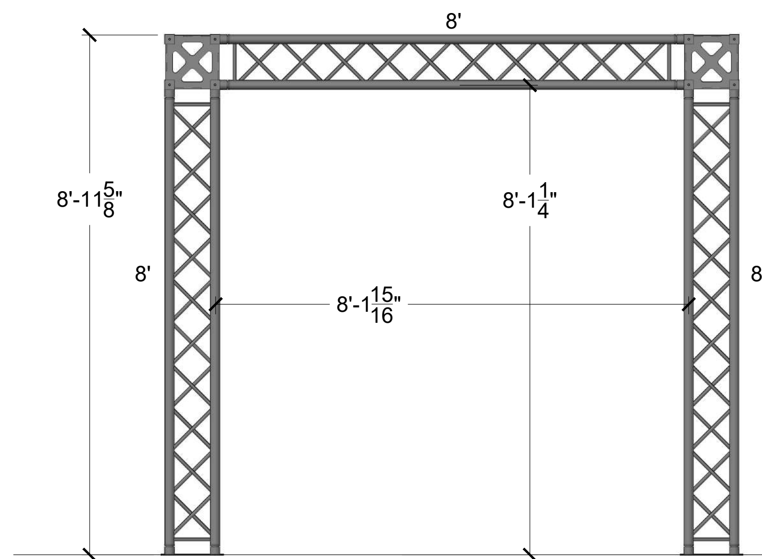
FRONT ELEVATION
