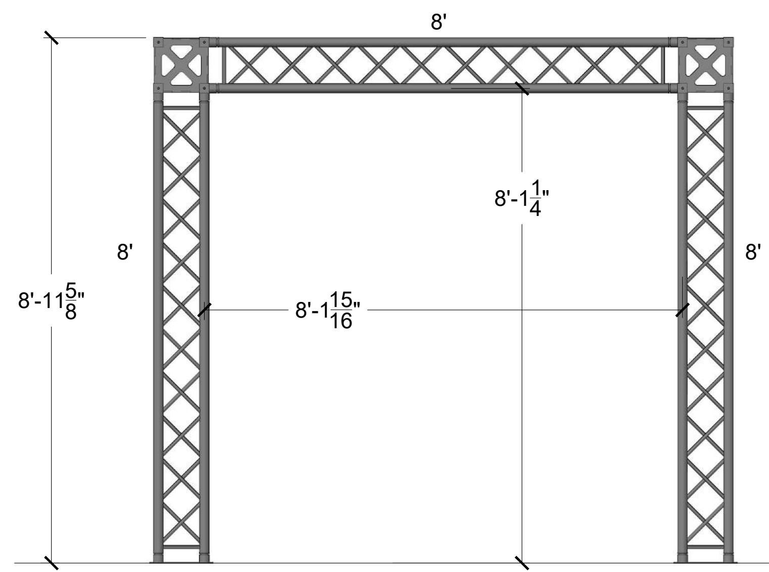
FRONT ELEVATION
