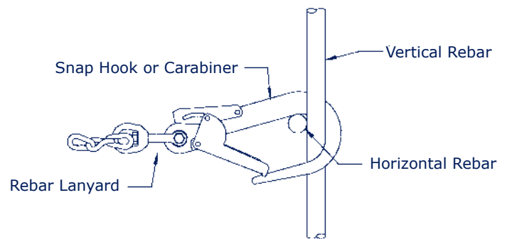
Figure 6 - Connecting To The Anchorage
