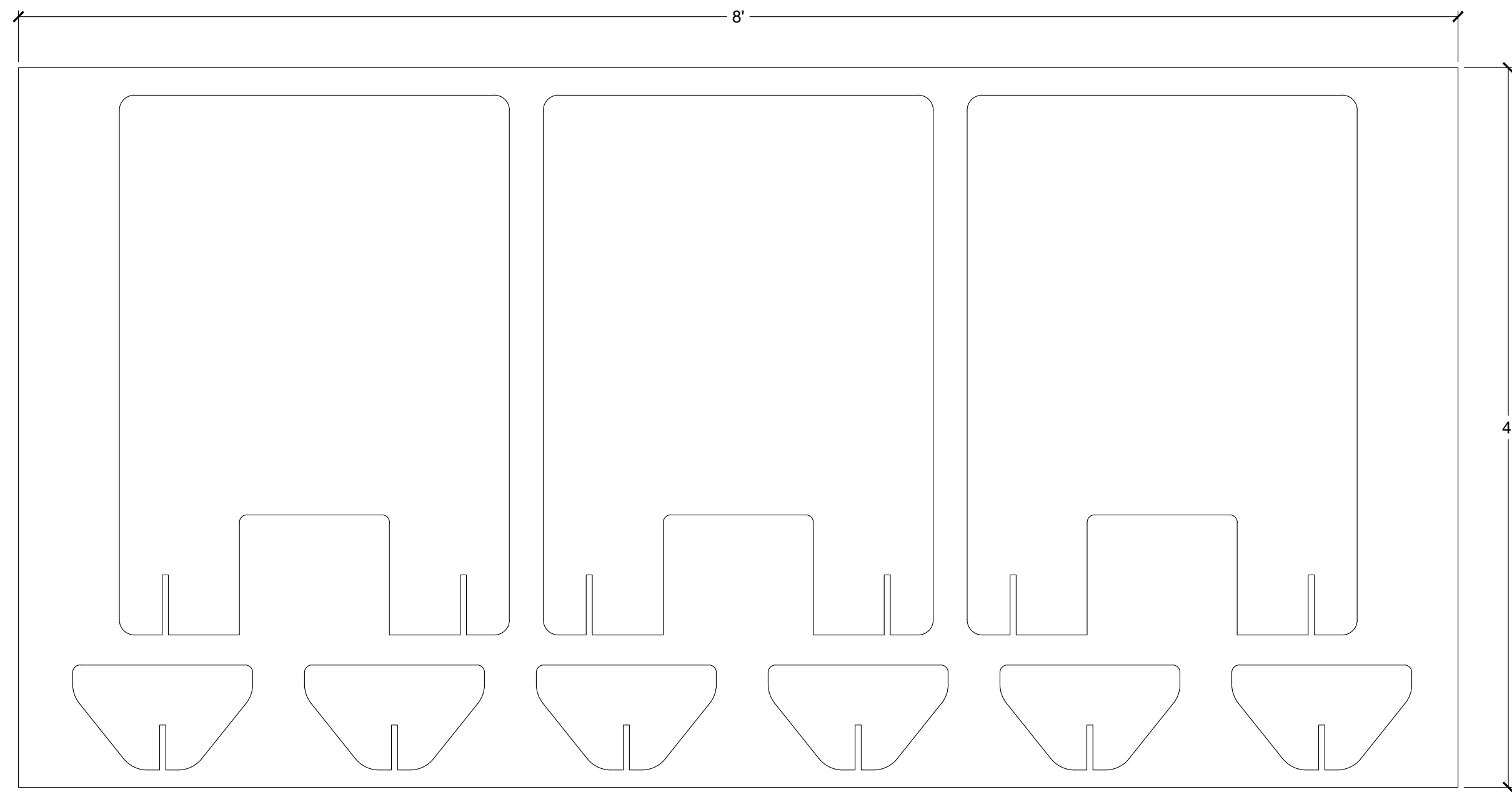
SNEEZE GUARD - PLEXI LAYOUT - CUT FROM 3/8" CLEAR PLEXI SCALE: 1-1/2" = 1'-0"
