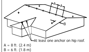
Figure 5 - Anchor Locations
