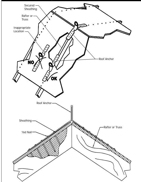
Figure 7 - Anchor Installation
