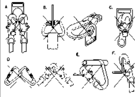
Figure 4 - Inappropriate Connections
