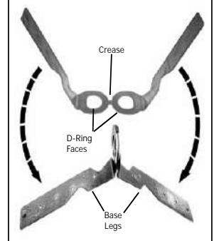
Figure 6 - Anchor Preparation
