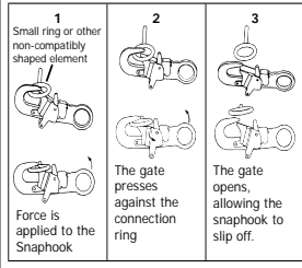
Figure 4 - Inappropriate Connections
