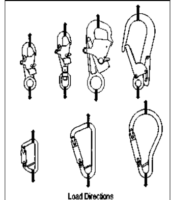
Figure 8 - Load Direction
