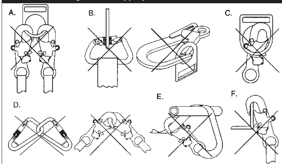
Figure 3 - Inappropriate Connections
