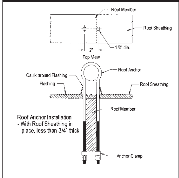
Figure 11 - Roof Anchor Installation
