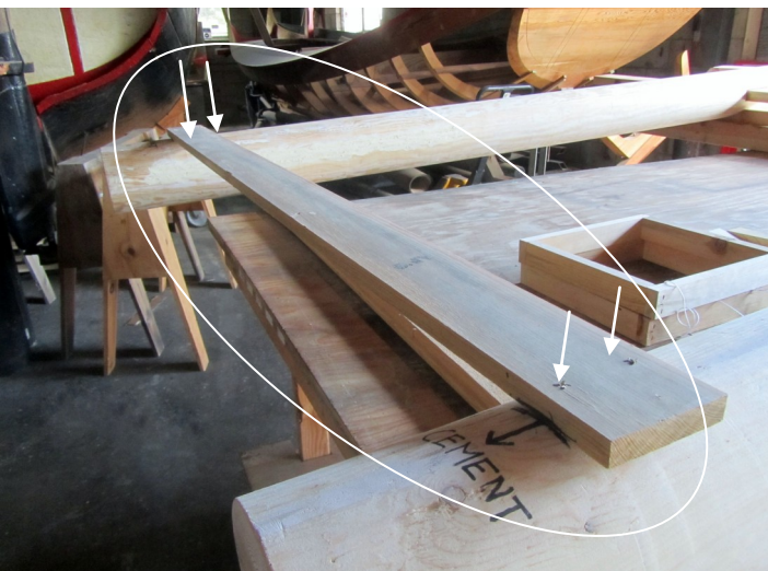
11. Fasten a temporary wood board with large screws where marked.
