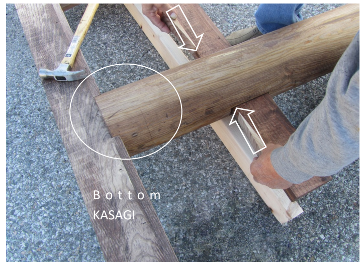
12. Insert two KUSABI into a hole to fill the gap.
