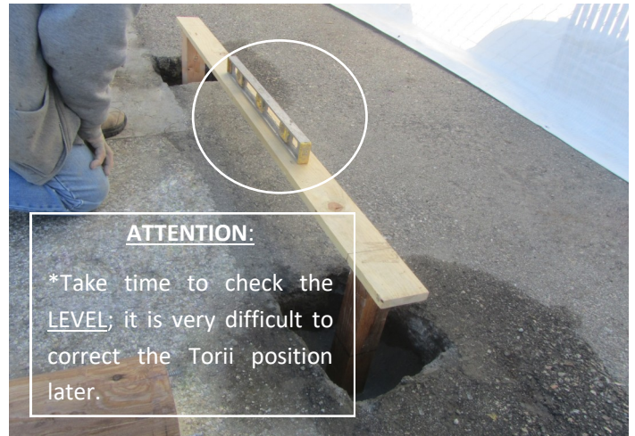
2. Place two wood blocks in the holes. Put an extra wood board at top to check the level; it will facilitate the Torii installation. Remove the wood blocks.
