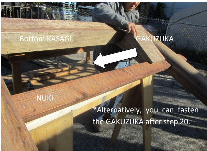
9. Fit two GAKUZUKA (wider side at top) between the bottom KASAGI and NUKI and fasten them with small screws.
