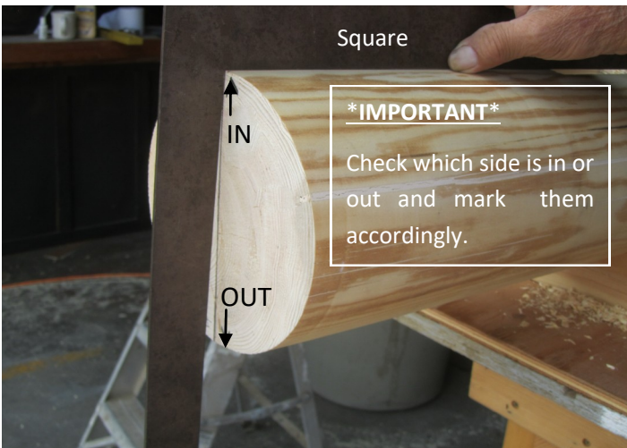
3. Place poles with a hole at top and check which side is in or out with a square; Torii poles are slightly inclined outward and mark OUT for a short side and IN for the other.
