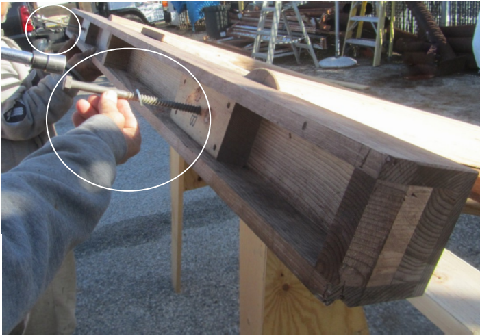
7. Fasten the bottom KASAGI and the HASHIRA poles with lag bolts from top.
