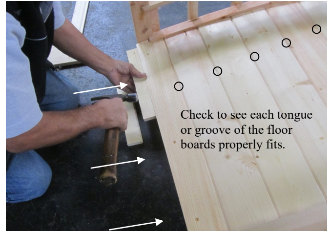
16. Turn over the end floor board and gently hammer it over an extra piece to tighten the fit.
