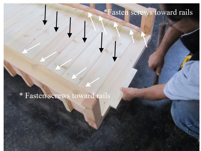
18. Slide in the end floor board, gently hammer it over an extra piece to tighten the fit, and fasten the end floor board with small screws .
