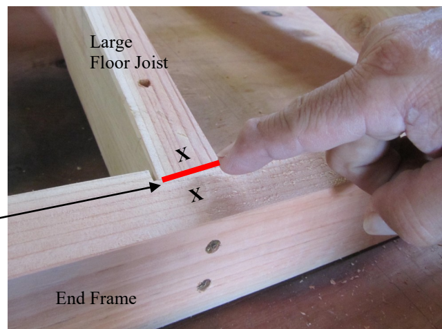
6. Be sure to set the end frame flush with the large floor joist (See "X").
