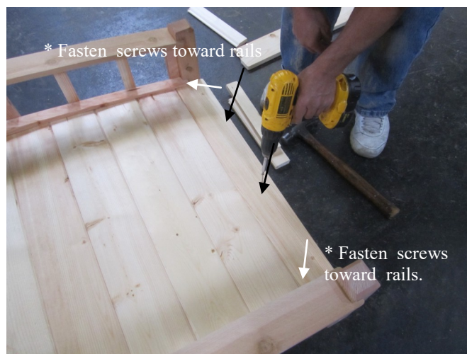
17. Fasten the end floor board with small screws .
