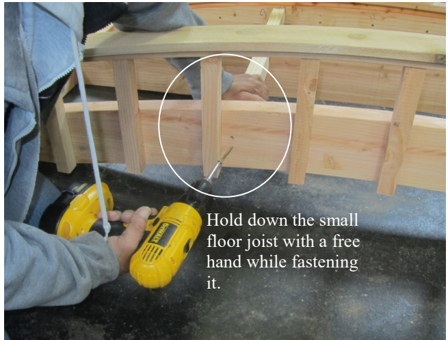
10. Do the same for the other side.
