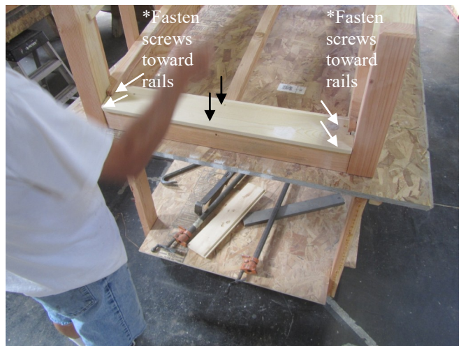
12. Turn it over and fasten it with small screws.
