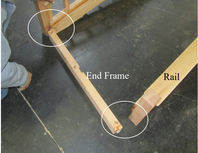
1. Start assembling two rails and two end frames. Match the number for the optimal result.
