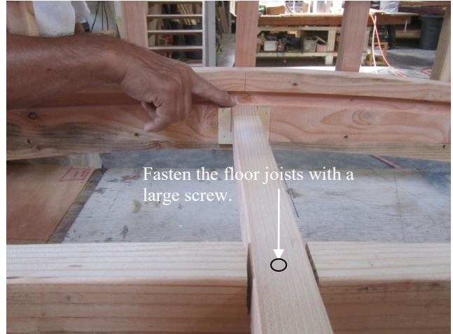
8. Fasten the floor joists with a large screw.
