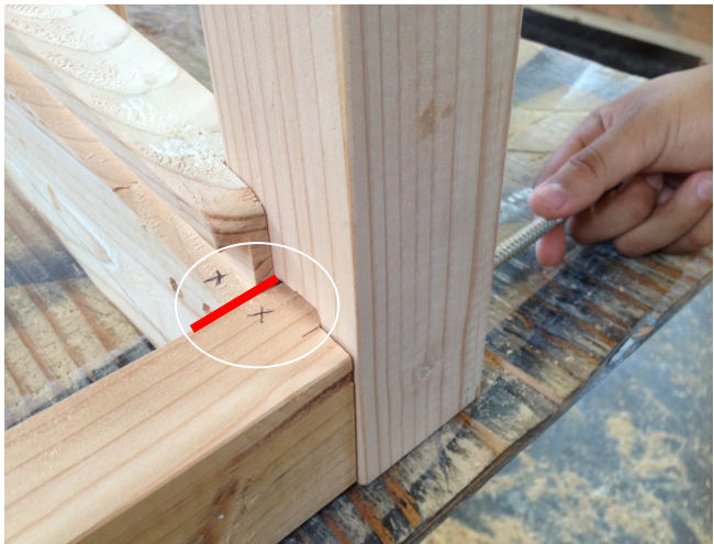
3. Be sure to set the end of the rail and end frame flush (See "X"). Do the same on three other sides.
