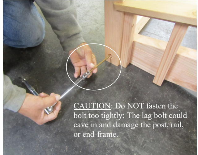
2. Fasten the rail and end frame with a large lag bolt .
