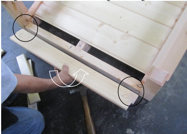
15. Put the end floor board. Match the number.
