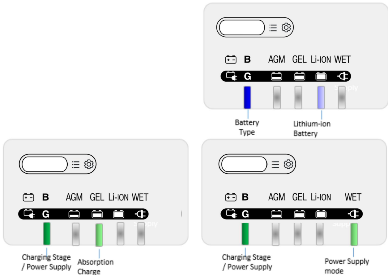
Figure 5-2 BS1210
