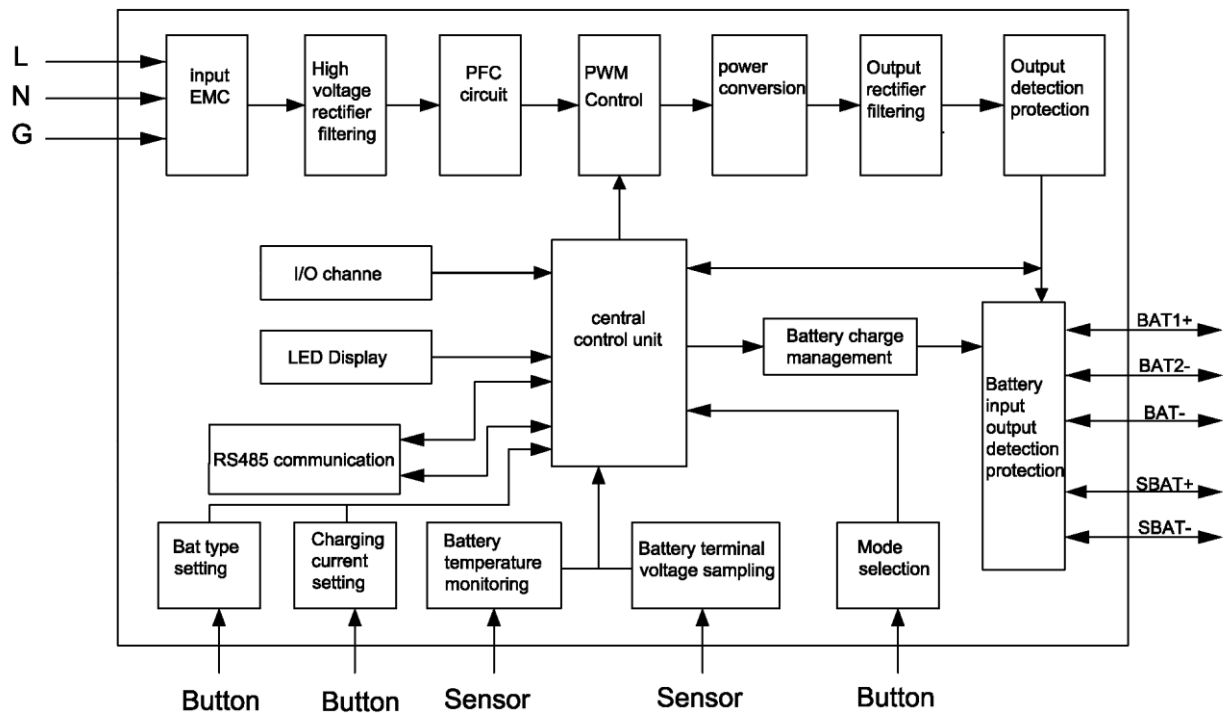
Figure 2-1 schematic diagram
