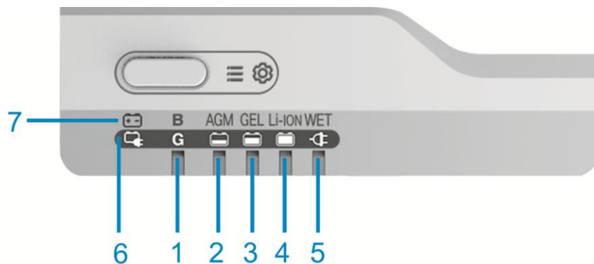
Figure 4-2 BS1210
