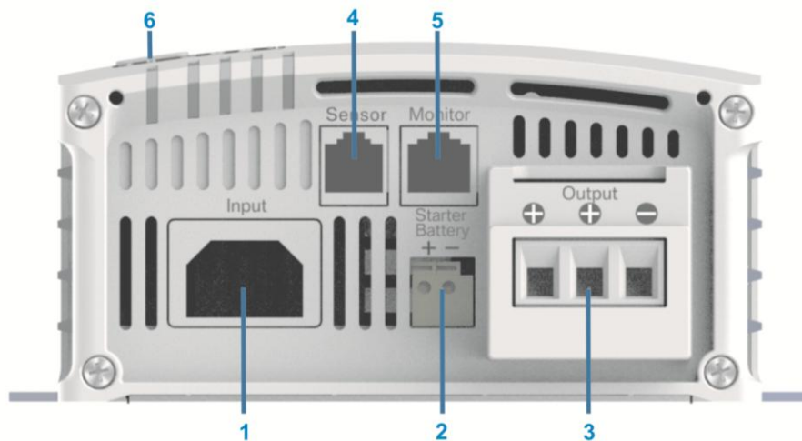
Figure 4-3 BS1225/BS1225-3/BS1240/BS1240-3/ BS2412/BS2412-3/BS2420/BS2420-3
