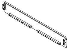
E. Lower Back Rail x 1 Barra Trasera Inferior
