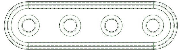
KK. Metal Plate x2 Plaque de métal # 1536
