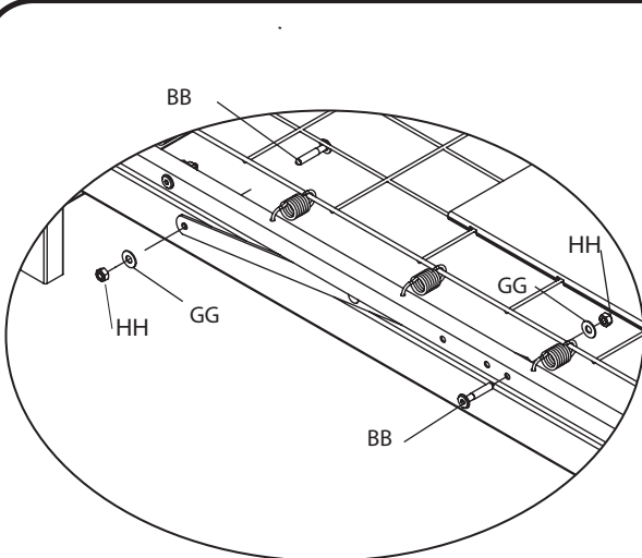
GG. - (8) Flat Washer Rondelle plate Arandela plana
