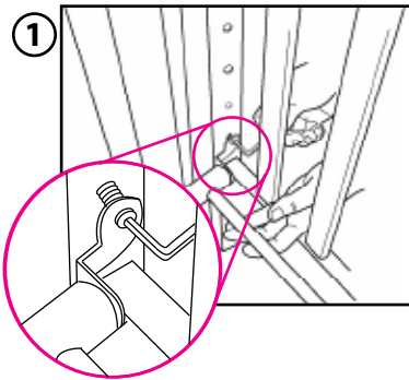
1 Remove mattress support from crib. Figure 1.
