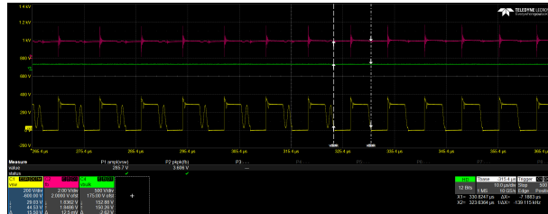
Figure 8-2. 1st and 2nd Valley Operation at 115VAC
