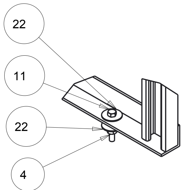
DETAIL G SCALE 0.350
