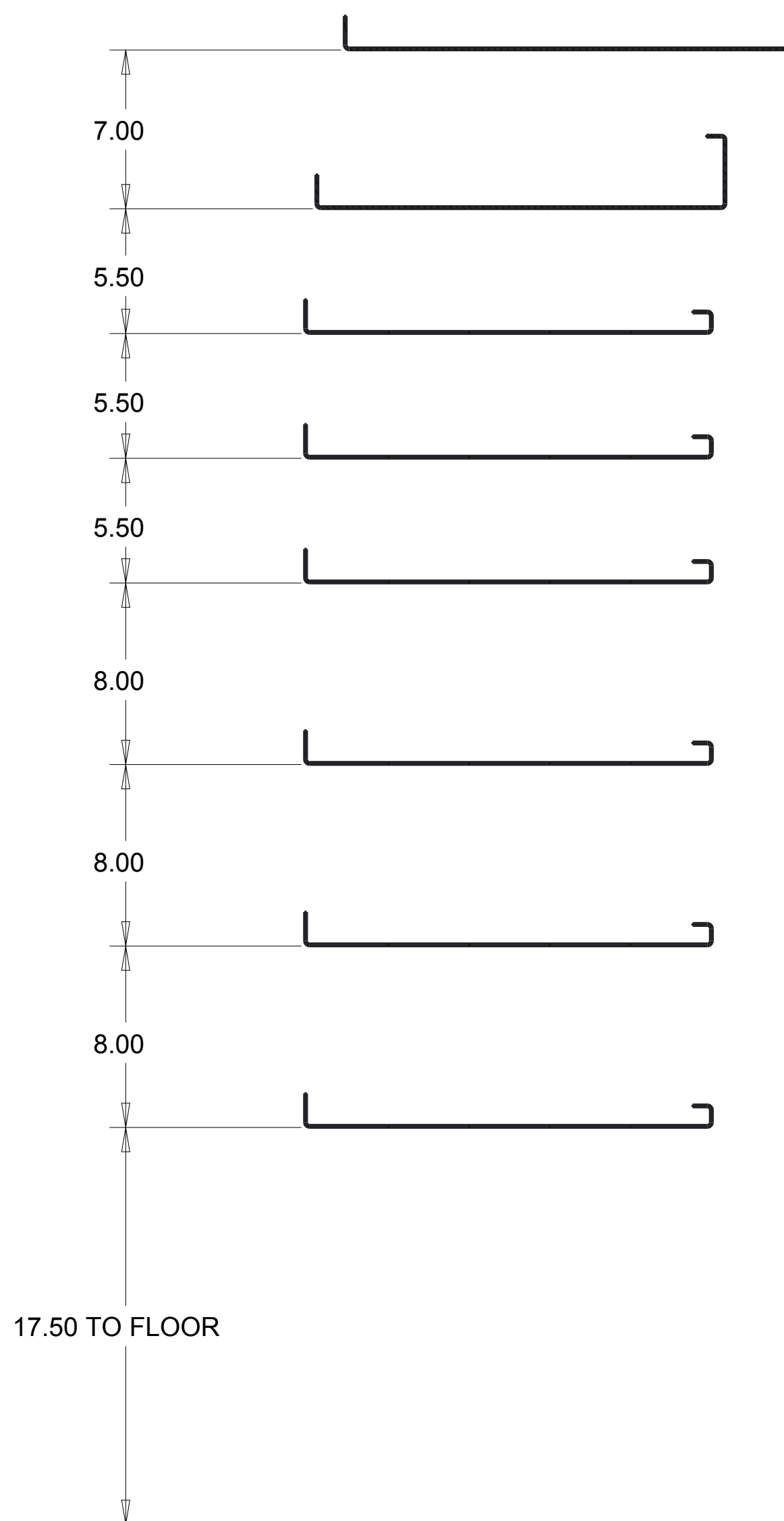
SECTION B-B SCALE 0.175
