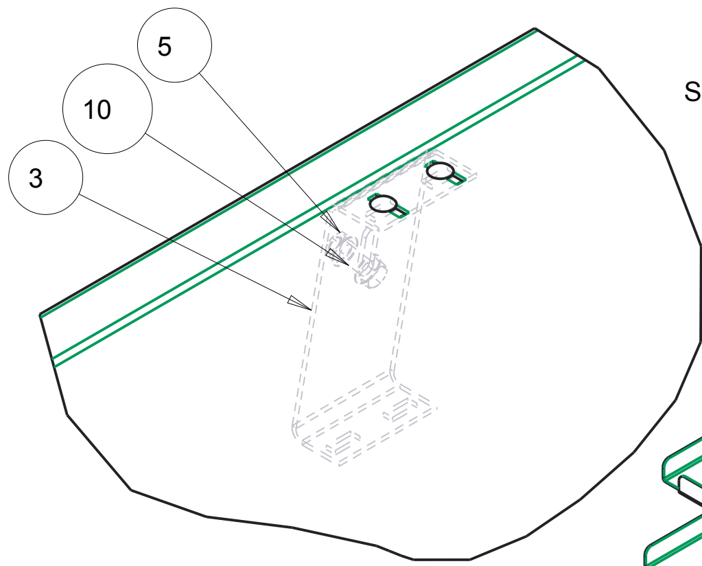
DETAIL F SCALE 0.350
