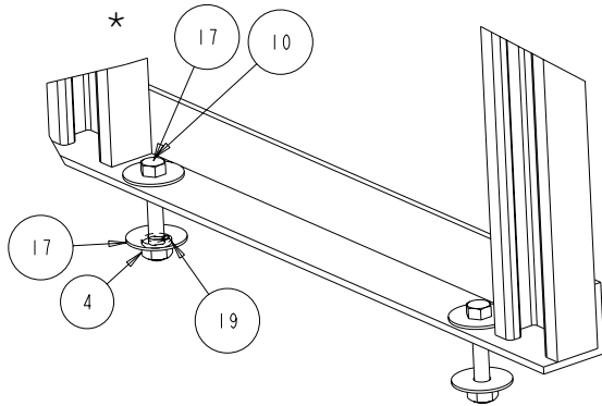
DETAIL E SCALE 0.650 BOLT THRU FLOOR
