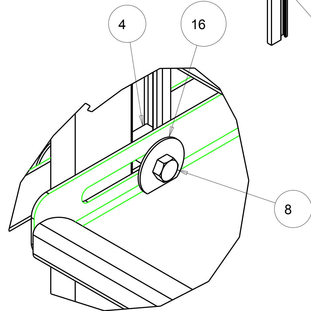
DETAIL A SCALE 0.750
