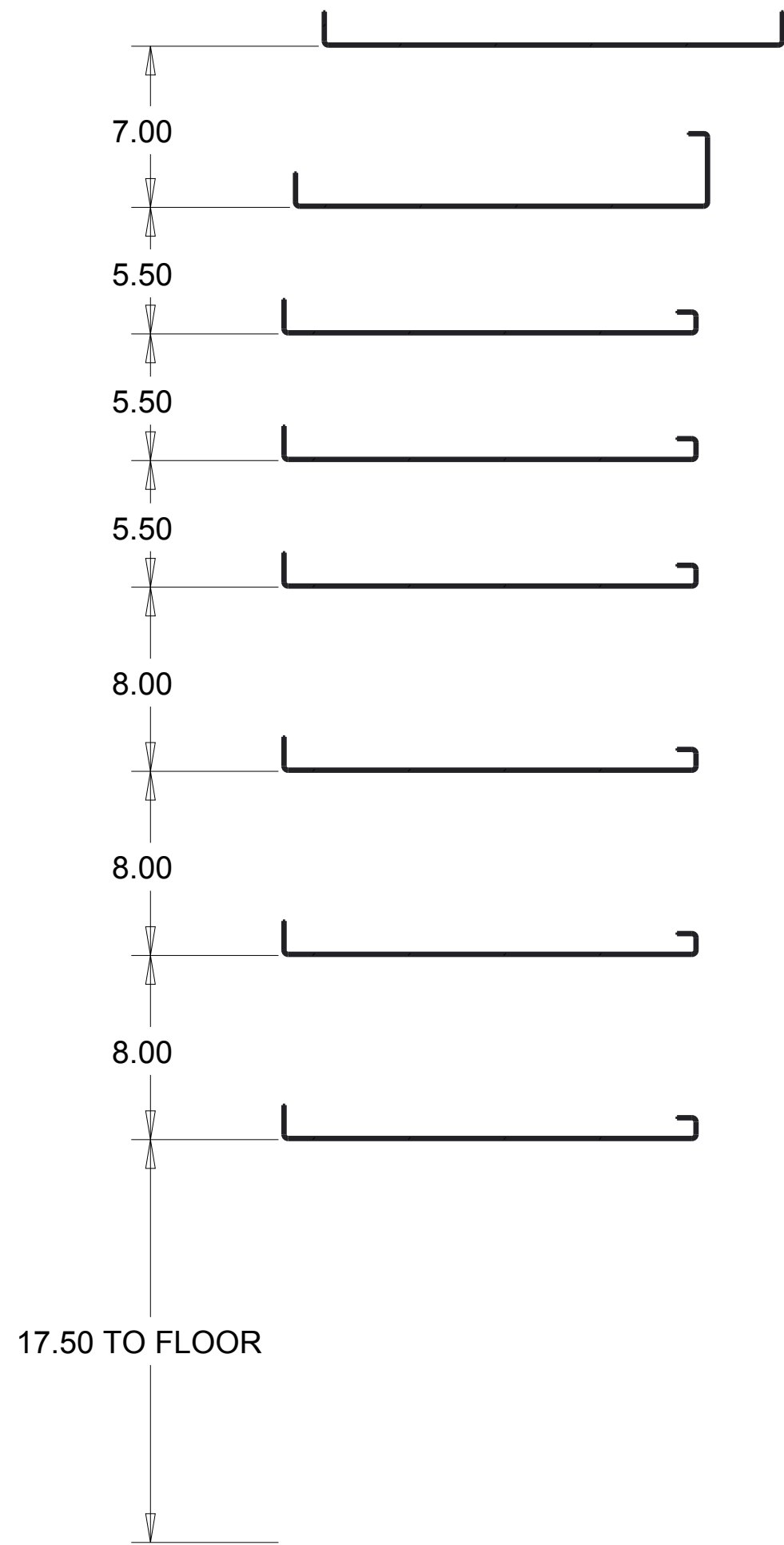
SECTION B-B
