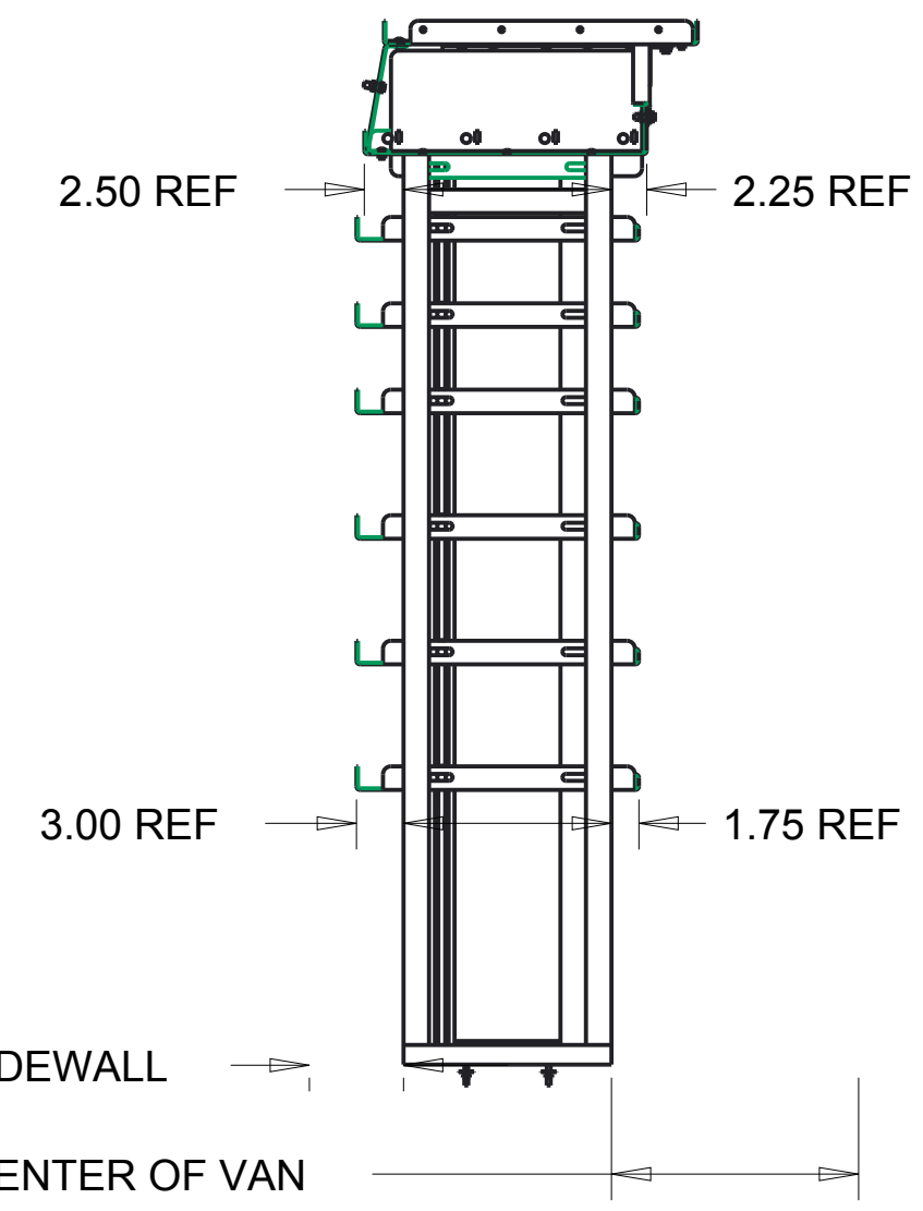
VIEW FROM REAR OF VAN
