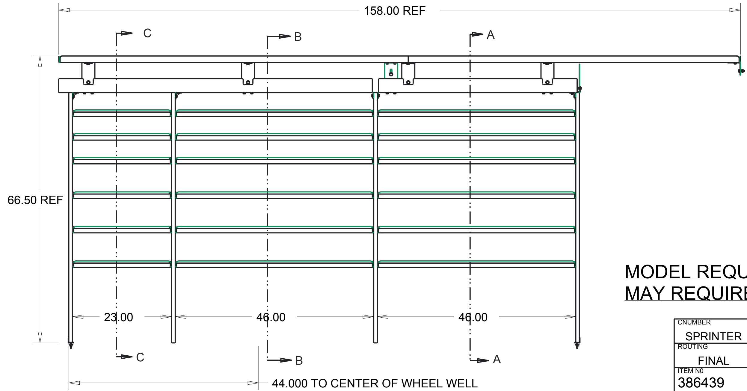
VIEW FROM AISLE
