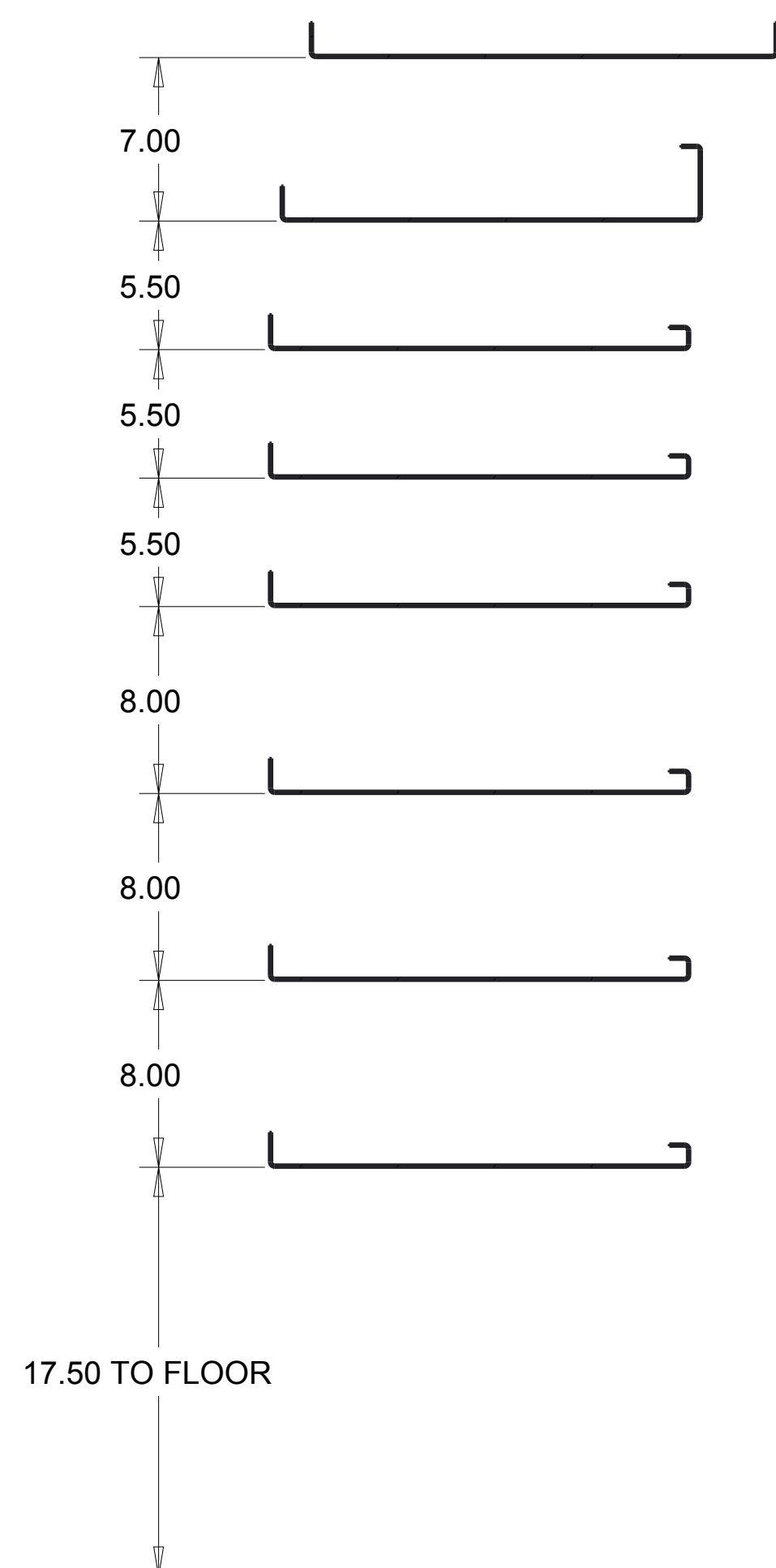
SECTION C-C
