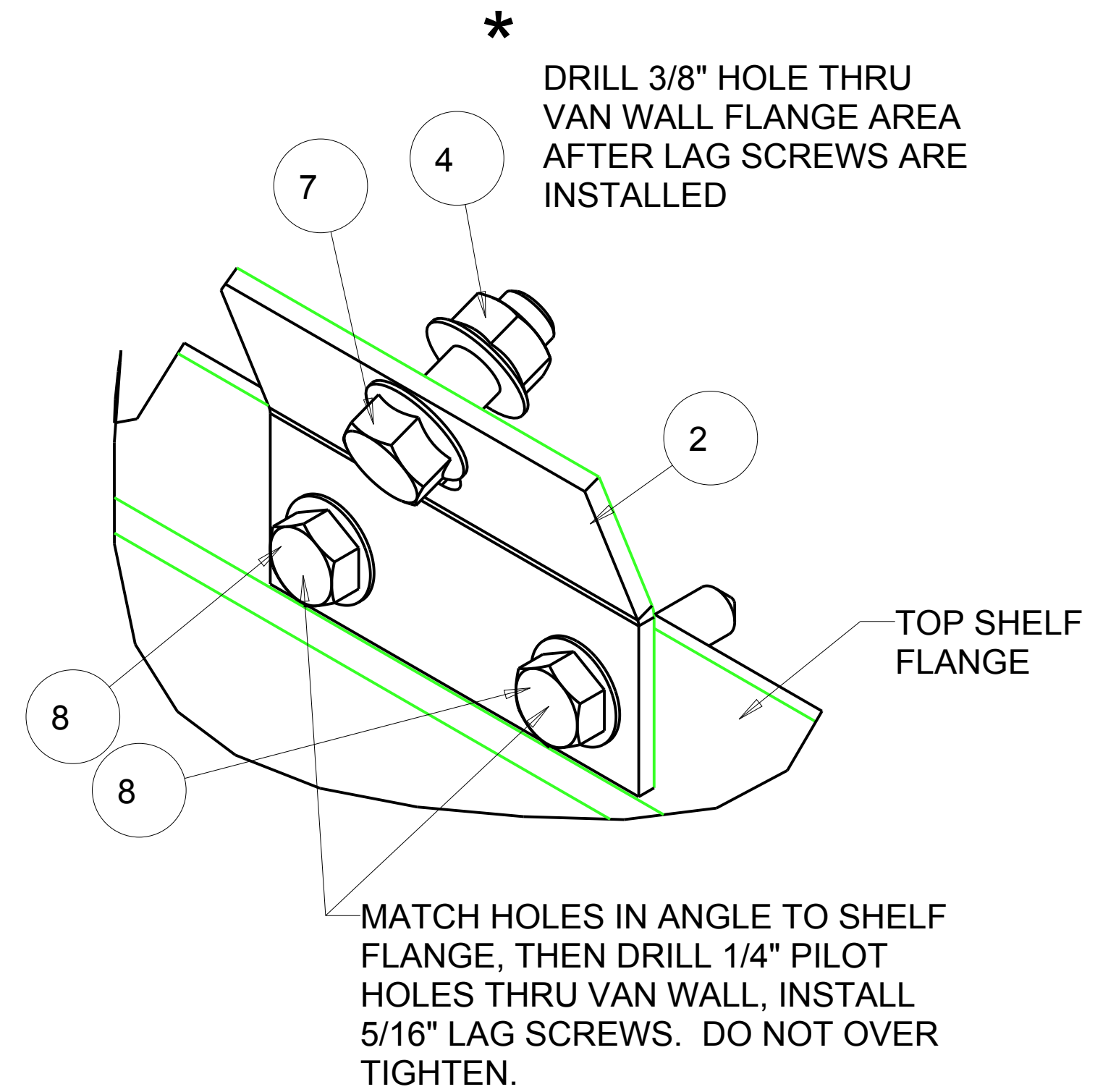
DETAIL B SCALE 1.250
