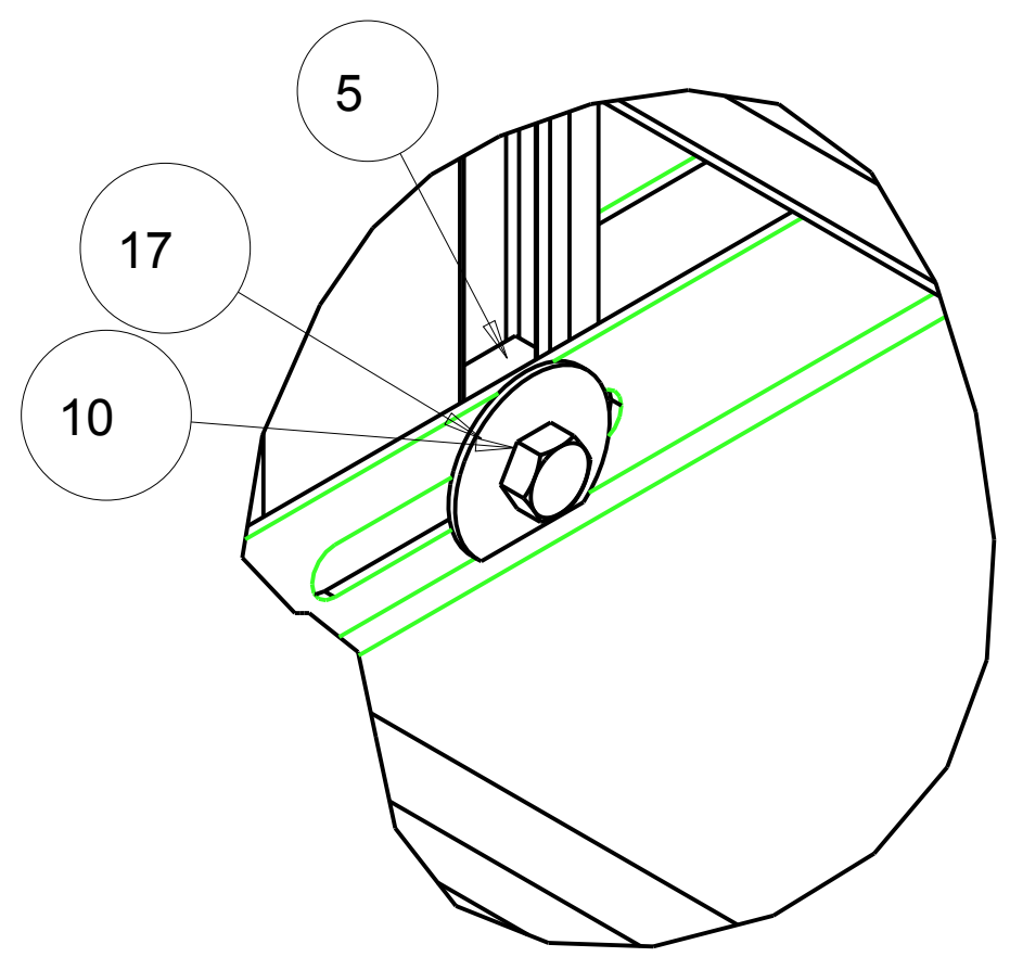
TYP. SHELF HARDWARE DETAIL C SCALE 0.700
