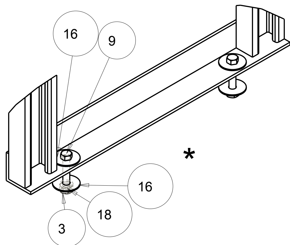
DETAIL D SCALE 0.500 BOLT THRU FLOOR
