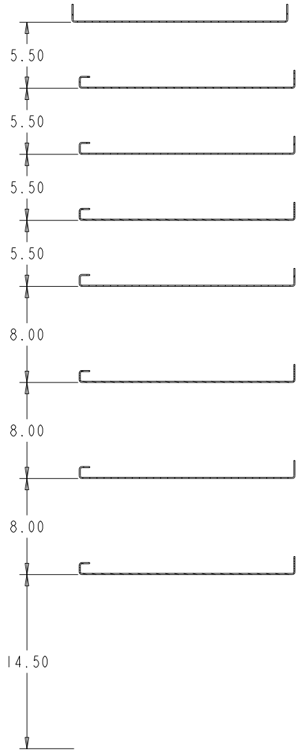
SECTION B-B
