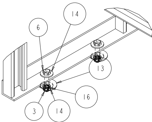
DETAIL D SCALE 0.500 BOLT THRU FLOOR
