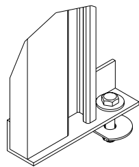
DETAIL E SCALE 0.500 BOLT THRU FLOOR
