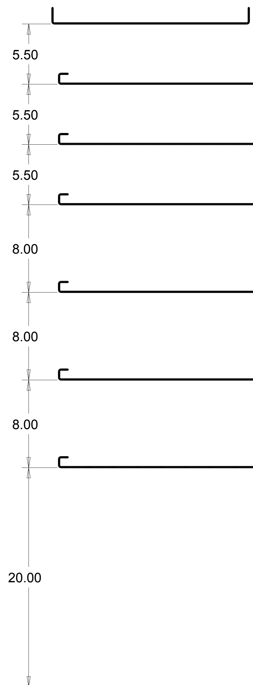
SECTION B-B
