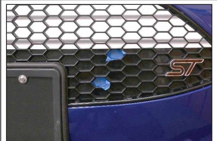
Mark the centers of the hexes shown above. Use assembled light plate to locate holes on the other side.
