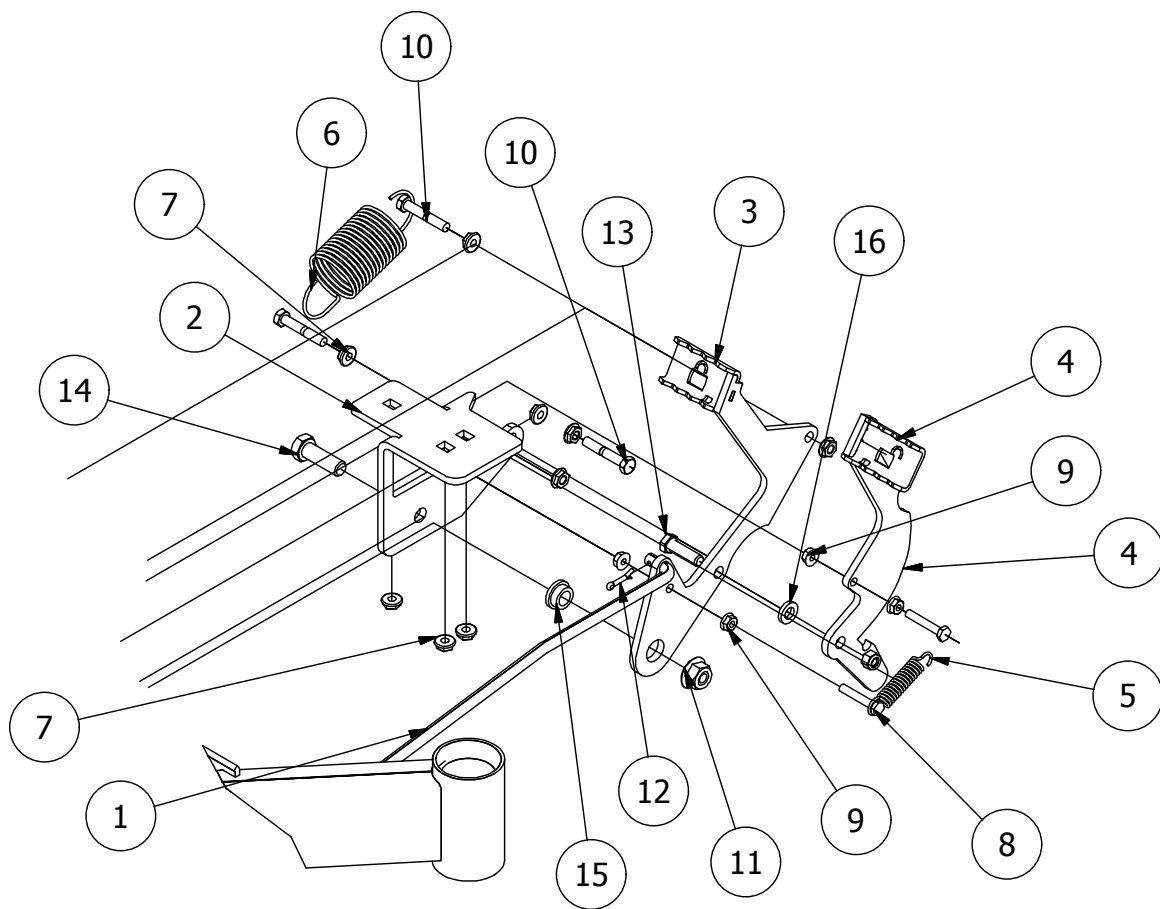
DETAIL A
