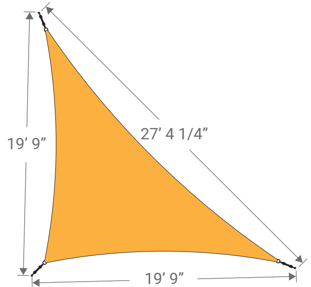
Minimum dimensions between attachment points for a tensioned sail with hardware
