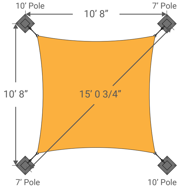
Dimensions from center-to-center of footings for optimal pole placement.
