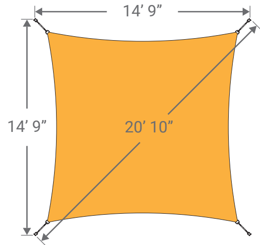
Minimum dimensions between attachment points for a tensioned sail with hardware
