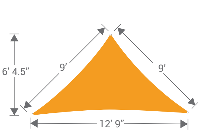
Dimensions of a relaxed sail
