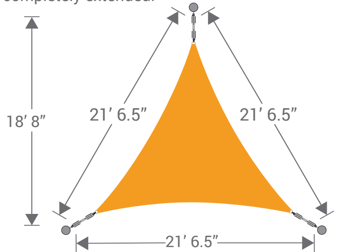
Minimum dimensions between anchor points for a tensioned sail with hardware
