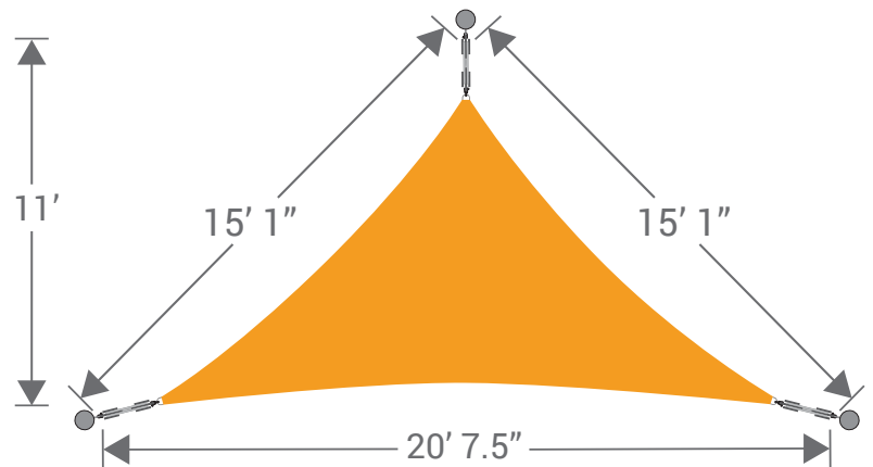
Minimum dimensions between anchor points for a tensioned sail with hardware
