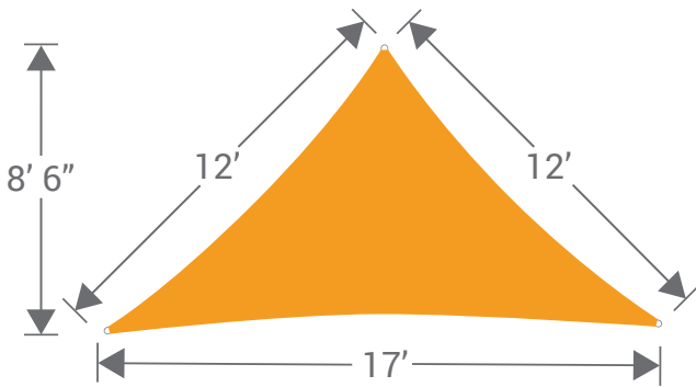
Dimensions of a relaxed sail
