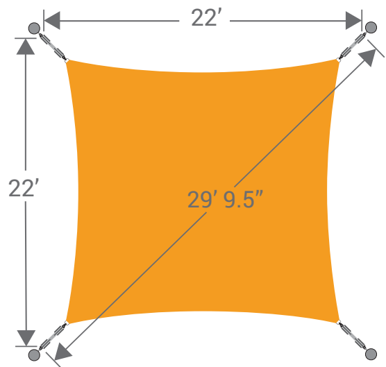
Minimum dimensions between anchor points for a tensioned sail with hardware
