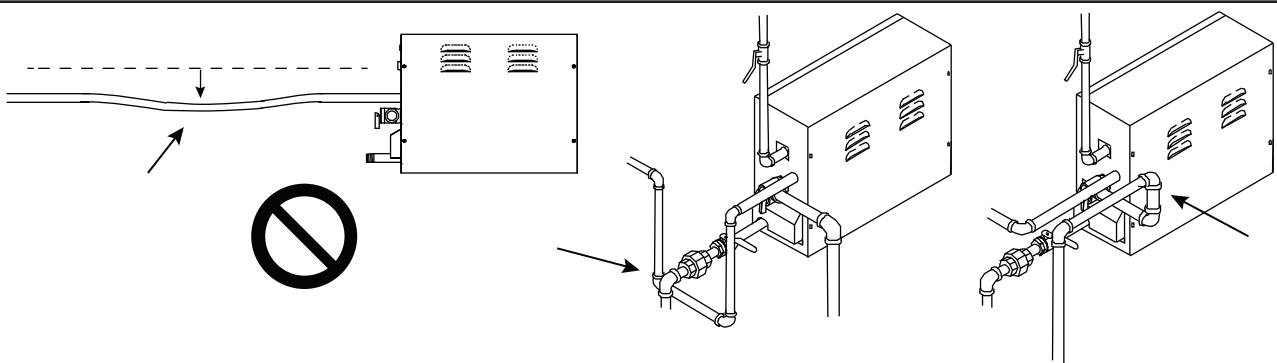
DIAGRAM 7: TYPICAL STEAM LINES
