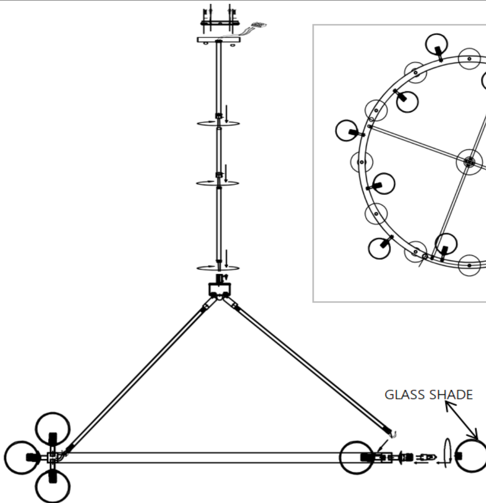
24PCS GLASS SHADE
