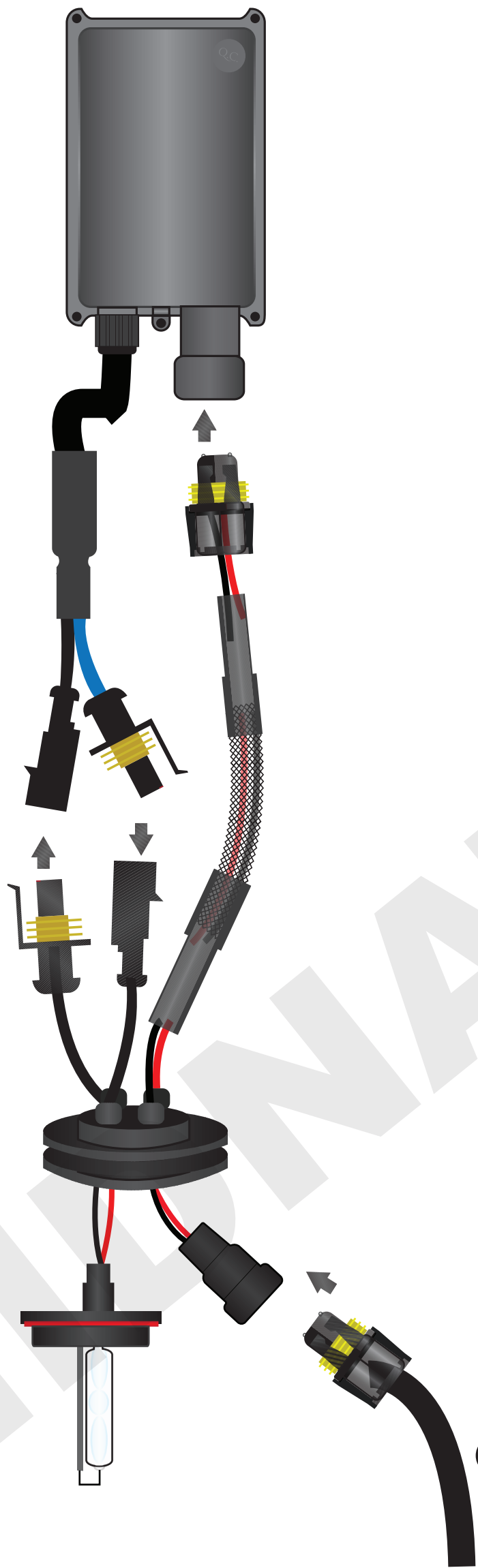
Car Factory Harness
