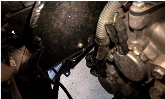
14. REMOVE 10MM (HEAD) BOLT PICTURED, INSTALL MAP INTAKE HEAT SHIELD USING PHILLIPS HEAD SCREWS AND BOLT YOU REMOVED EARLIER
