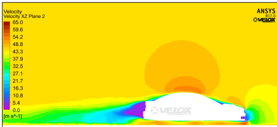
Figure 5.4.3: Velocity Plot XZ Plane 2 (Offset from Sym Plane 0.3m)
