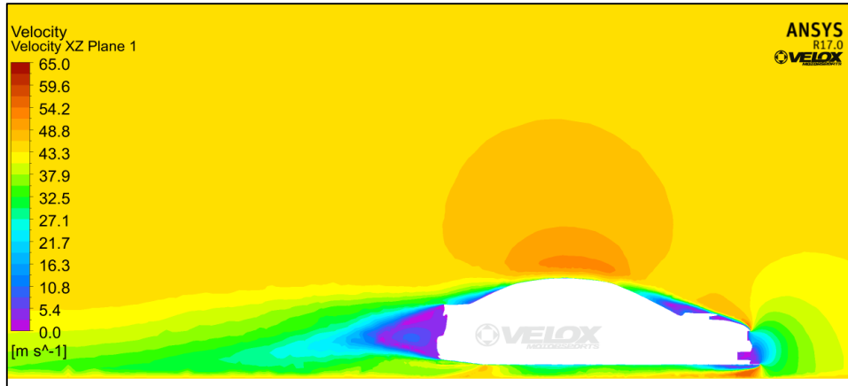
Figure 5.4.2: Velocity Plot XZ Plane 1 (Offset from Sym Plane 0.1m)
