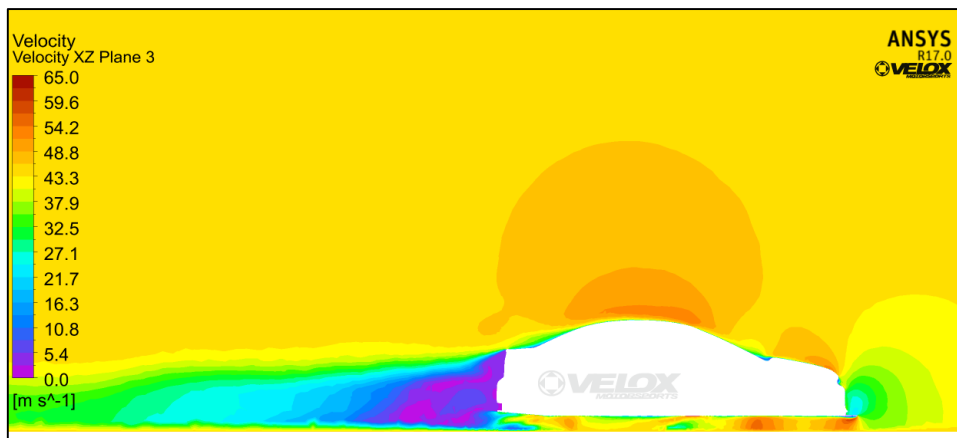
Figure 5.4.4: Velocity Plot XZ Plane 3 (Offset from Sym Plane 0.5m)
