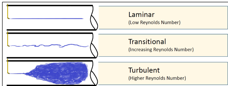
Figure 3.3.1: Flow Classifications
