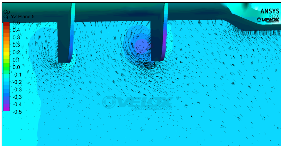
Figure 5.7.3: Vortex Formation on Strake
