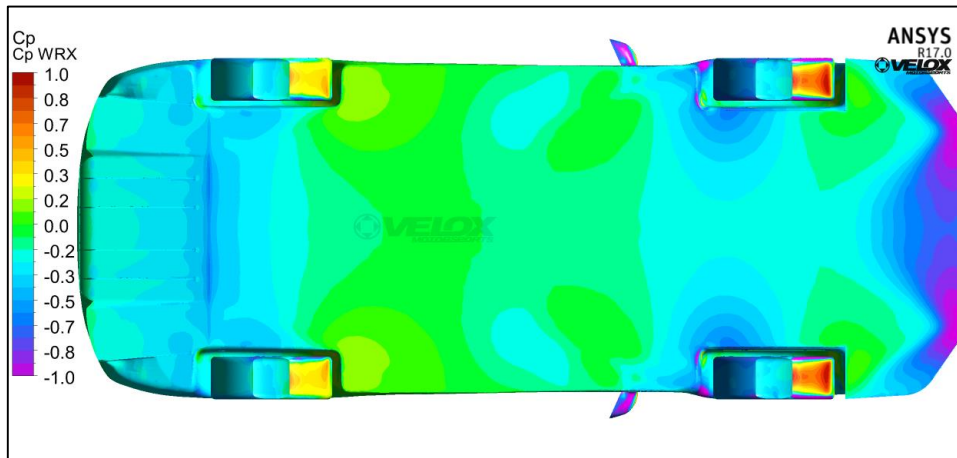
Figure 5.3.4: Cp Bottom
