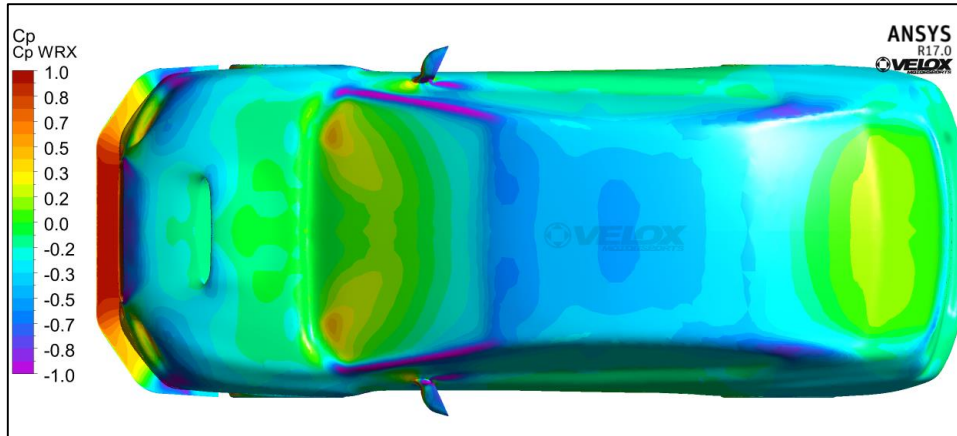
Figure 5.3.3: Cp Top
