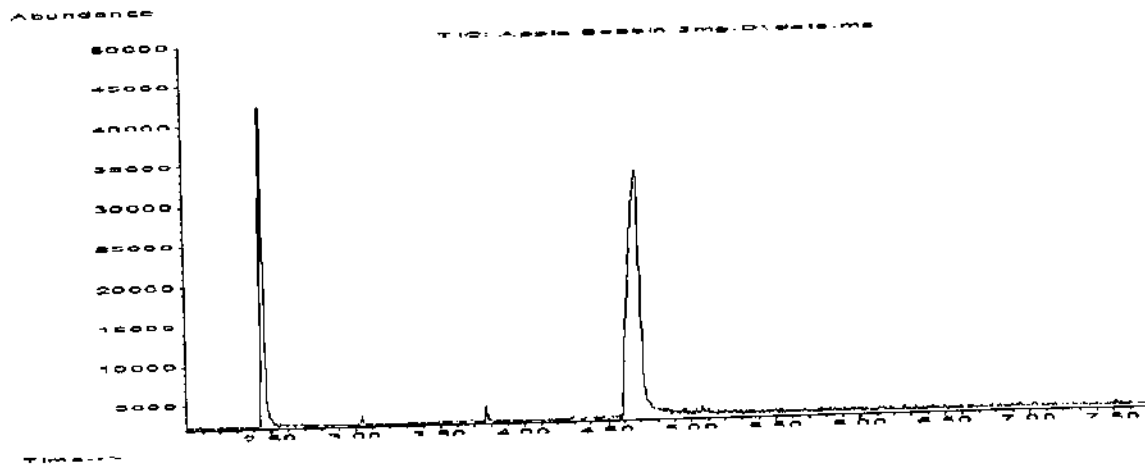
Figure 1. GC-MS Chromatogram of sample.
