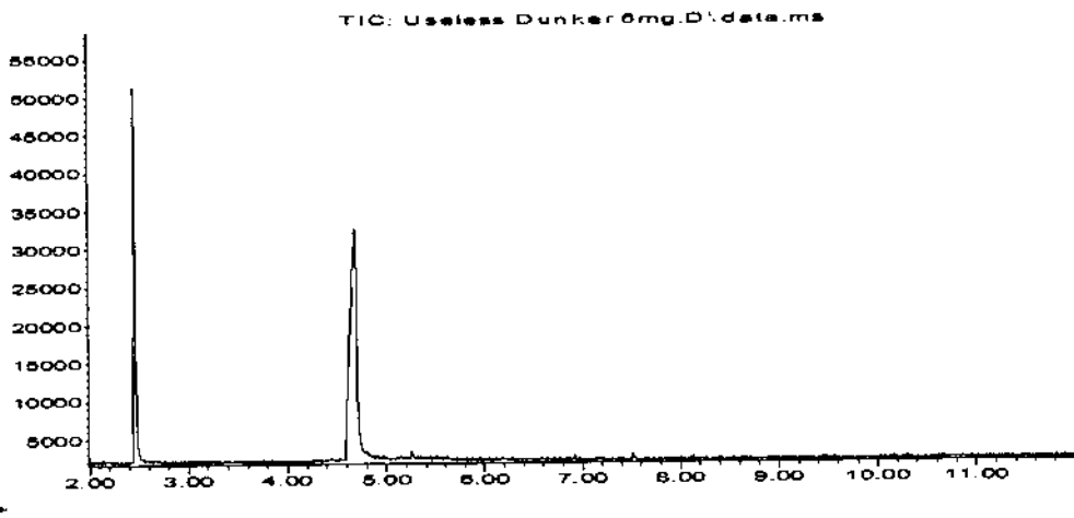
Figure 1. GC-MS Chromatogram of sample.
