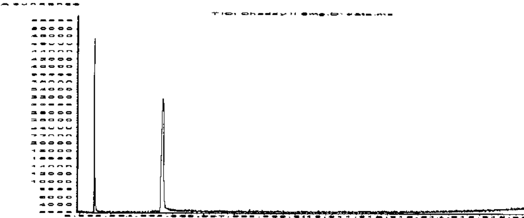
Figure 1. GC-MS Chromatogram of sample.
