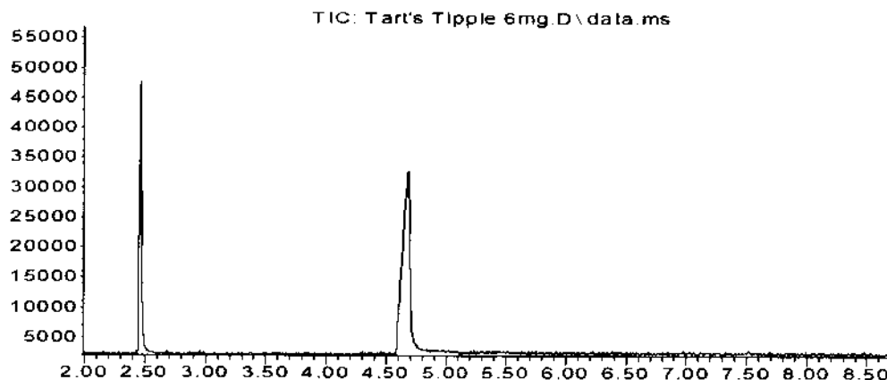
Figure 1. GC-MS Chromatogram of sample.
