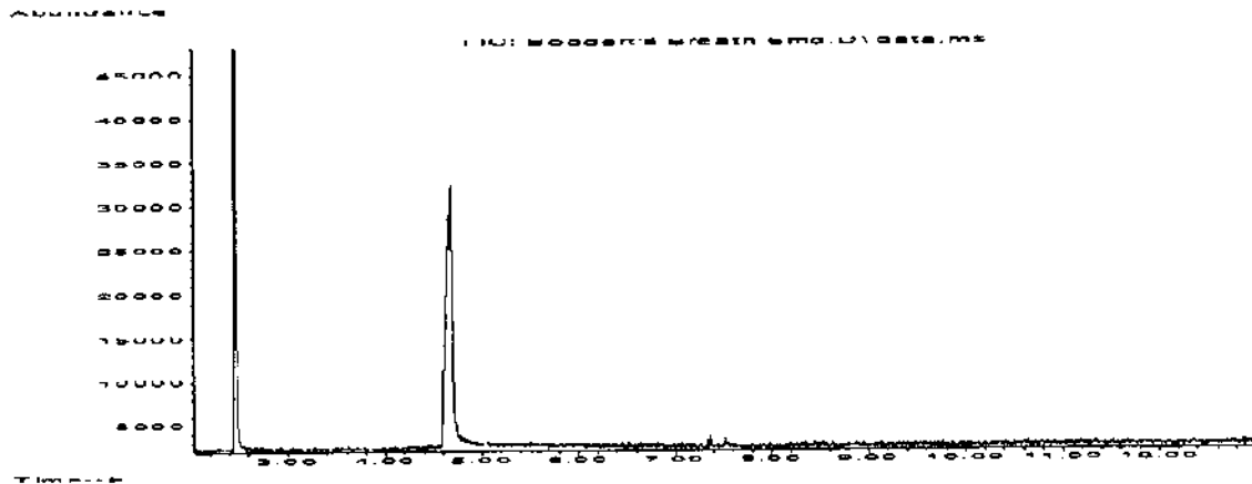
Figure 1. GC-MS Chromatogram of sample.
