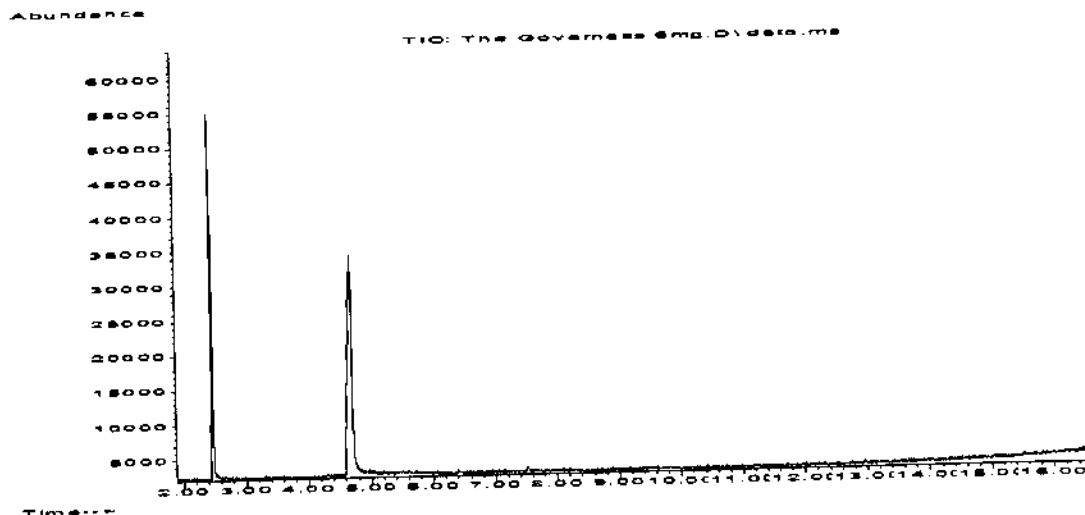
Figure 1. GC-MS Chromatogram of sample.
