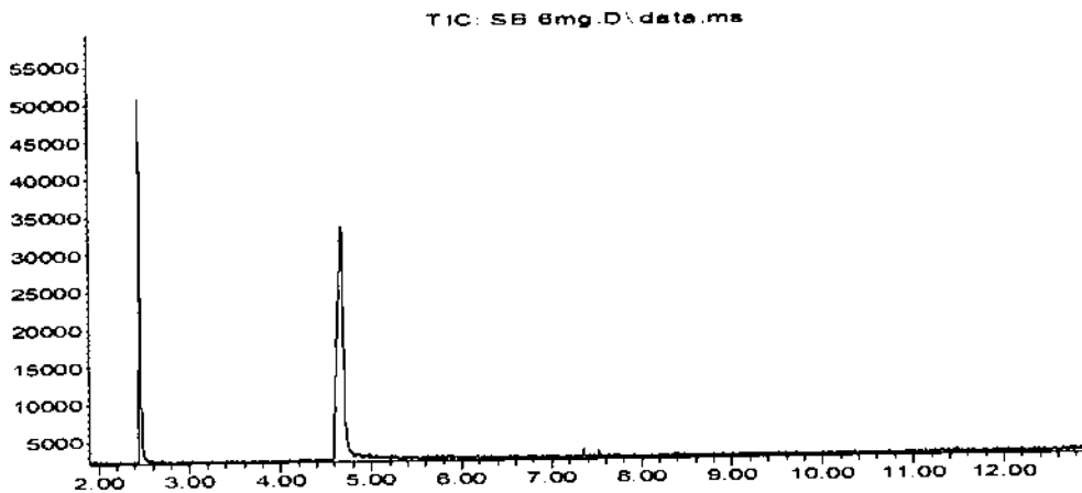
Figure 1. GC-MS Chromatogram of sample.
