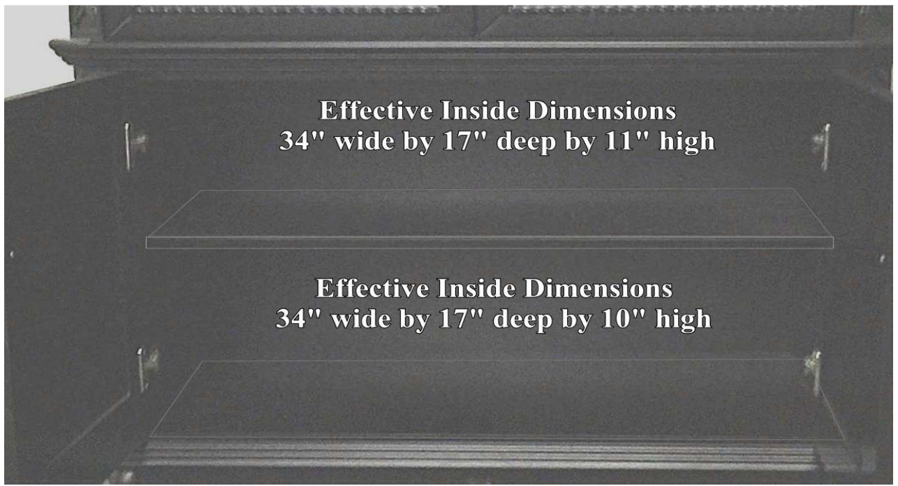
Effective Inside Dimensions of the two (2) Bottom Cabinets – the shelf is fixed.
