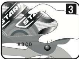
(A, B, C, D) KEEP PRESSING THE "PUSH" BUTTON AND ADJUSTING THE TOE CAP TO RIGHT POSITION (A, B, C, D)
