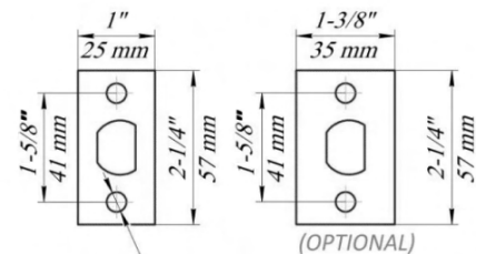
LATCH FACEPLATE
