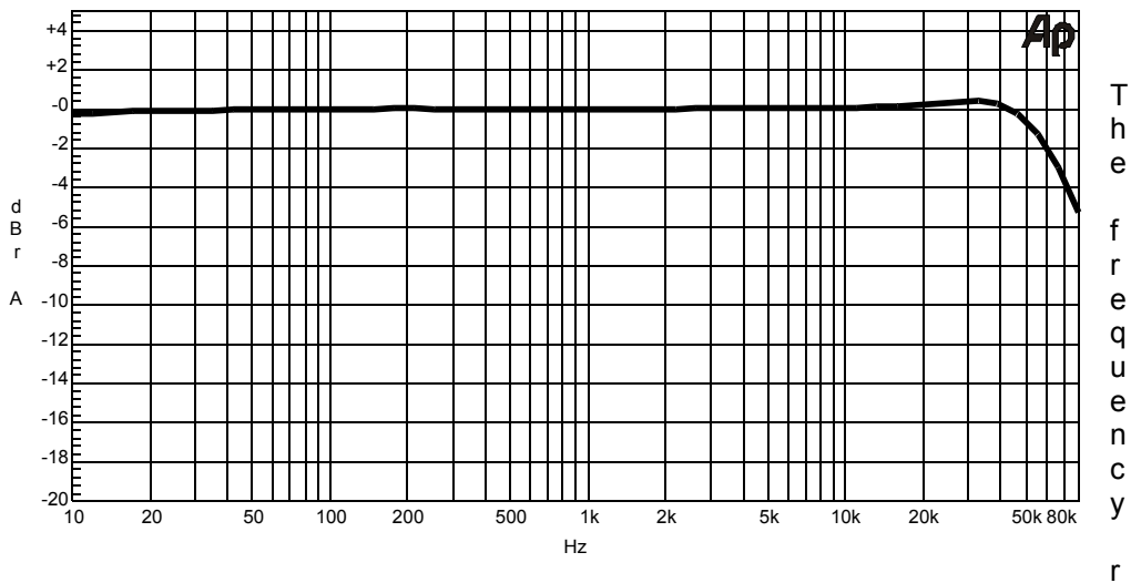
Graph 2: Frequency response, 4 V into 4 ohms
