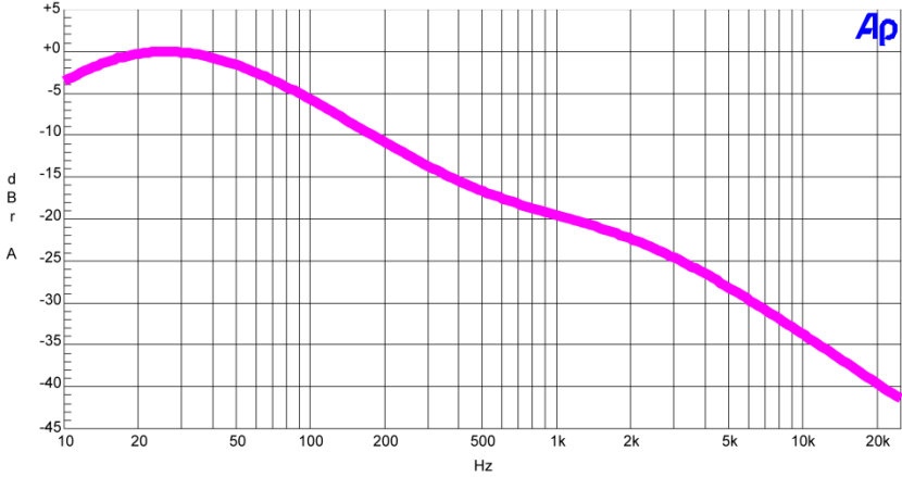
Frequency response with subsonic filter
