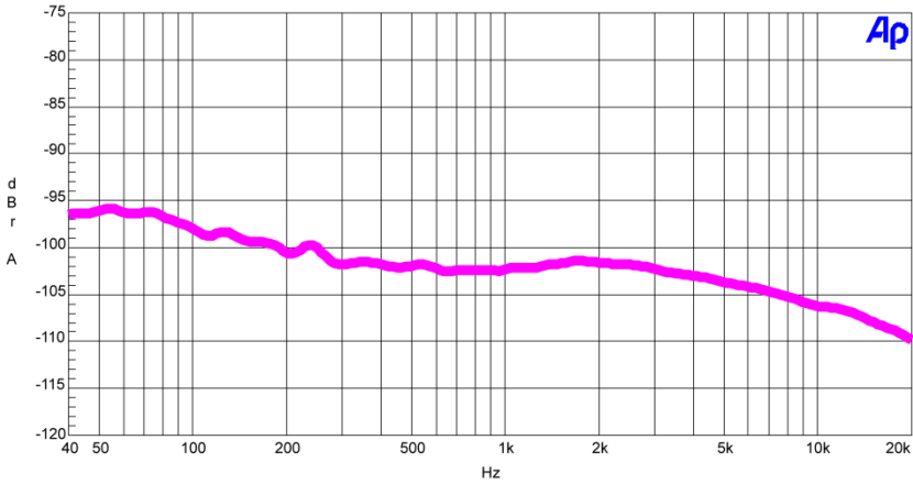
Hum and noise level with MC, gain = 58 dB
