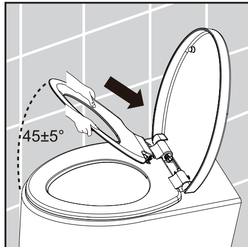
4. Hold the child seat to 45 \pm 5^\circ , then push and snap into place.
