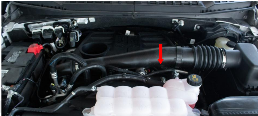
2018-2020 3.0L Powerstroke Charge Air Cooler Sensor Sensor is located on the top of the connector at the engine throttle body underneath the air intake tube.
